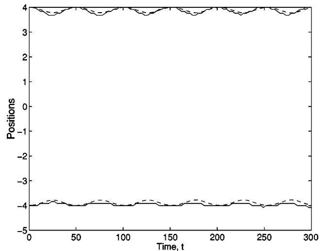
FIG. 2. Two-soliton interactions and their comparison with the CTC model. Solid curve, numerical results; dashed curve, predictions from the Toda chain model. \nu_1 = 0.95 , \nu_2 = 1.05 , \delta_1 = 0 , and \delta_2 = \pi .
